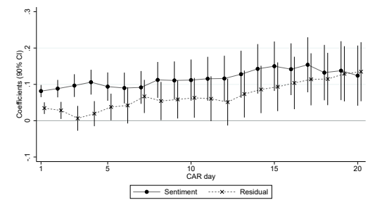
(c) New stock &amp; message selection
