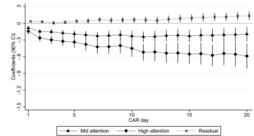
(f) New stock &amp; message selection
