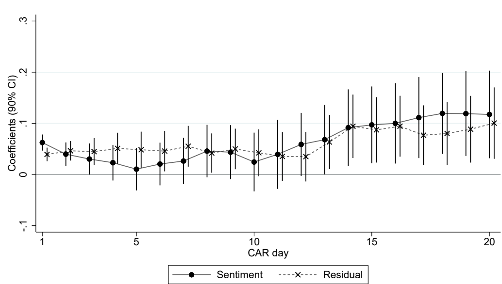
(a) Imbalance from sentiment v.s. from residual
