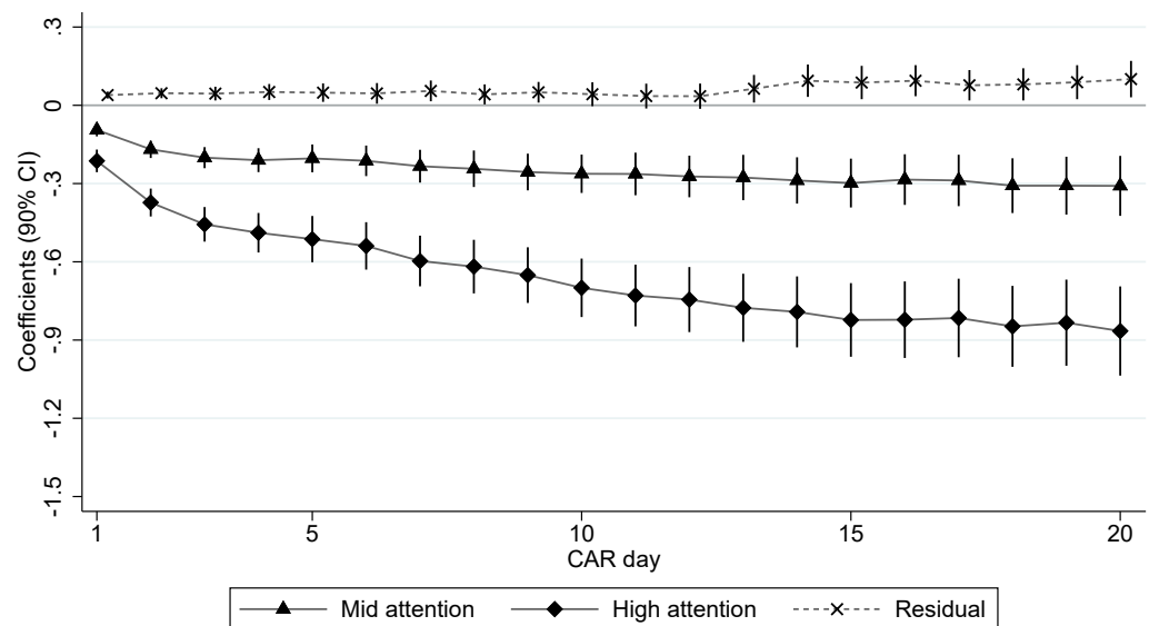
(b) Imbalance from attention v.s. from residual
